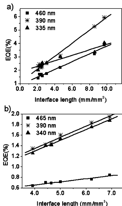
Figure 7. External quantum efficiency as a function of interface length for the excitation at the wavelength of the peaks of the absorption spectra of the homopolymers F8BT and PFB together with a linear fit. (a) 5:1 F8BT:PFB blend; (b) 1:5 F8BT:PFB blend.
